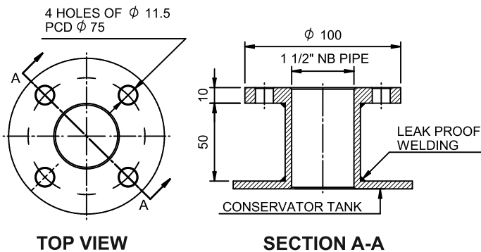
FIG 2. MOUNTING PAD
